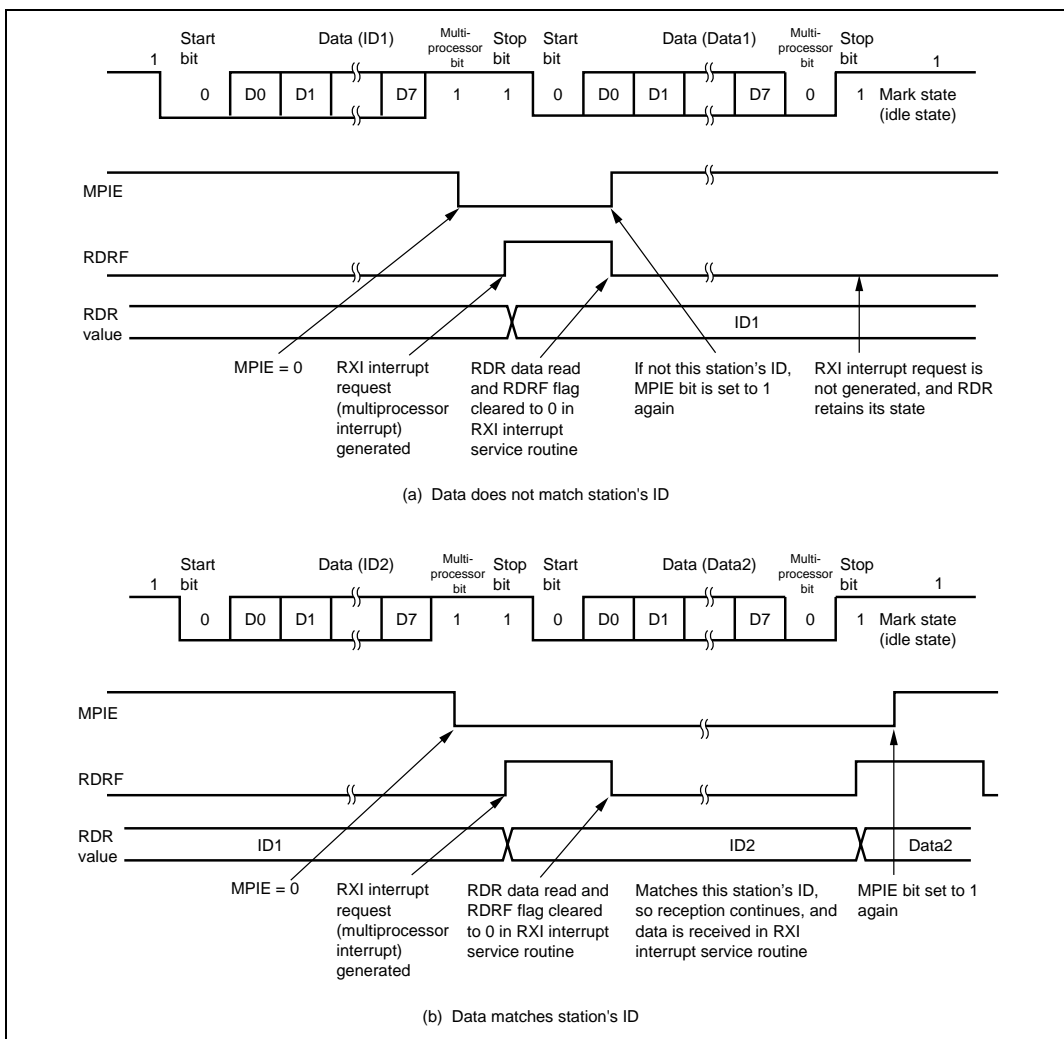
Figure 15.15 Example of SCI Operation in Reception (Example with 8-Bit Data, Multiprocessor Bit, One Stop Bit)
