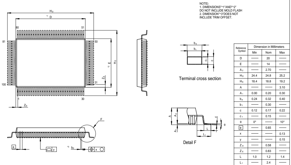
Figure C.3 FP-100A Package Dimensions
