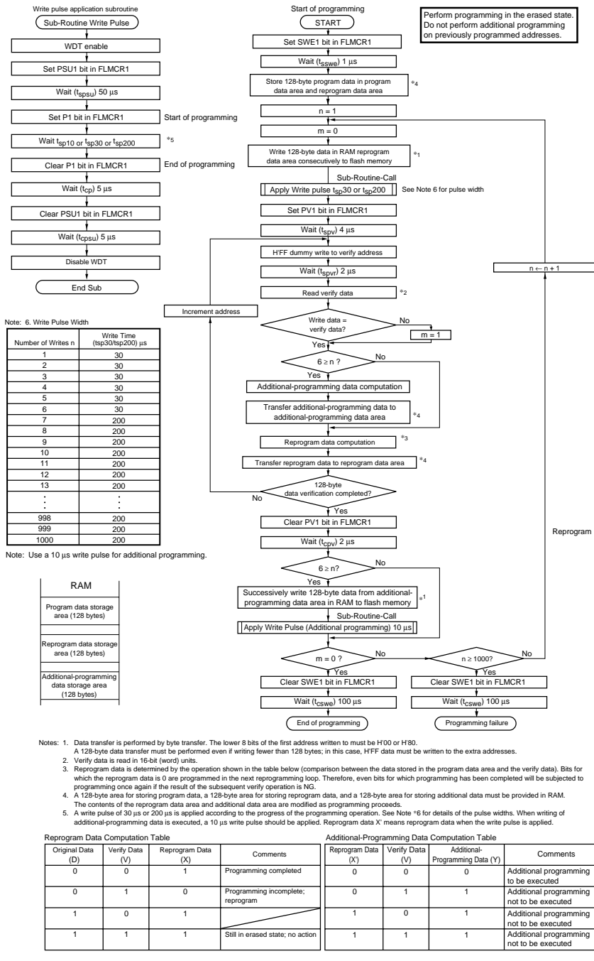
Figure 20.11 Program/Program-Verify Flowchart
